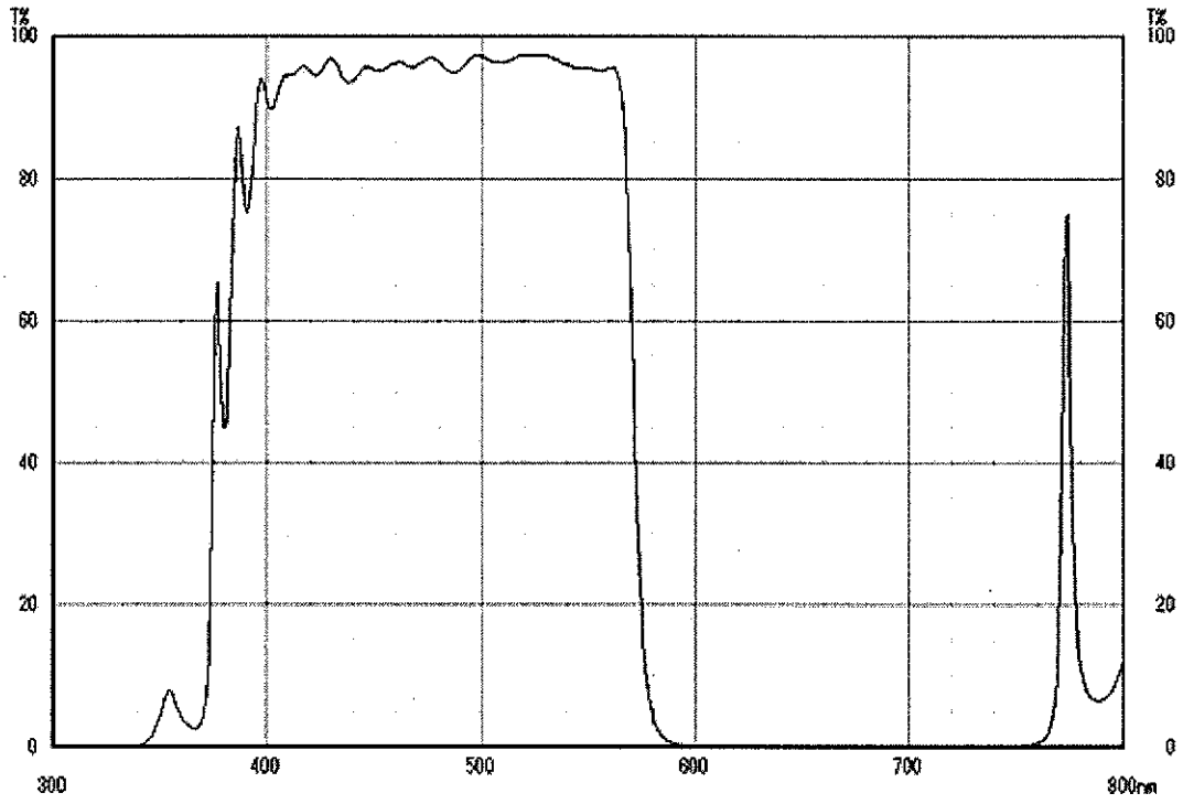
Short Wave pass filter
